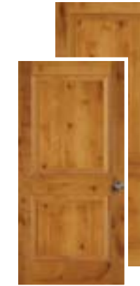
7282 ☉ 1-3/4" Fire-Rated 1-7/16" RP 6/8: 2/0, 2/4, 2/6, 2/8, 3/0 8/0: 1/6, 2/0, 2/4, 2/6, 2/8, 3/0, 3/6
