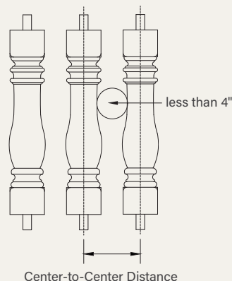
Straight Rail Application
