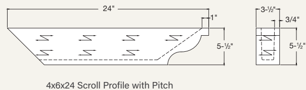
4x6x24 Scroll Profile with Pitch
