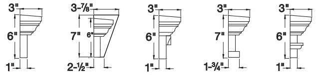
Standard w/ Keystone K6M w/ Dentil Trim w/ Bottom Trim 1 w/ Trim Strip
