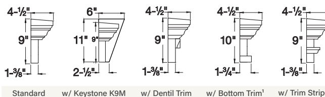
Standard w/ Keystone K9M w/ Dentil Trim w/ Bottom Trim¹ w/ Trim Strip
